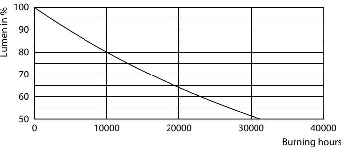
Lumen Maintenance Diagram - CorePro LEDbulb ND 4.9-40W A60 E27 840
