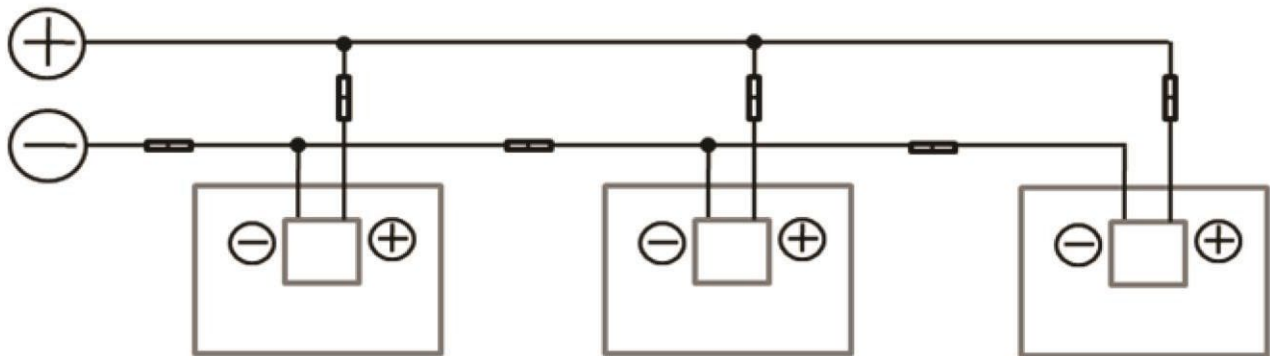
Parallel connection
