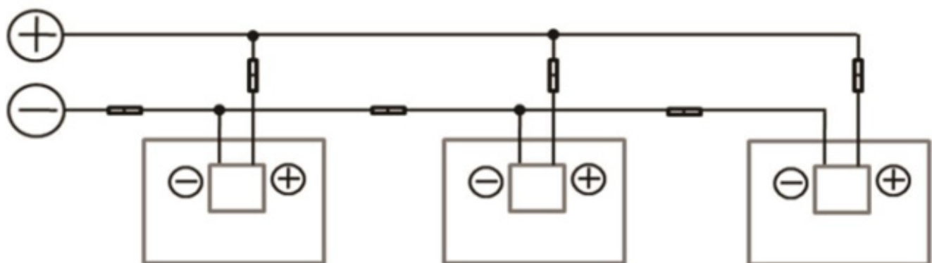
Parallel connection
