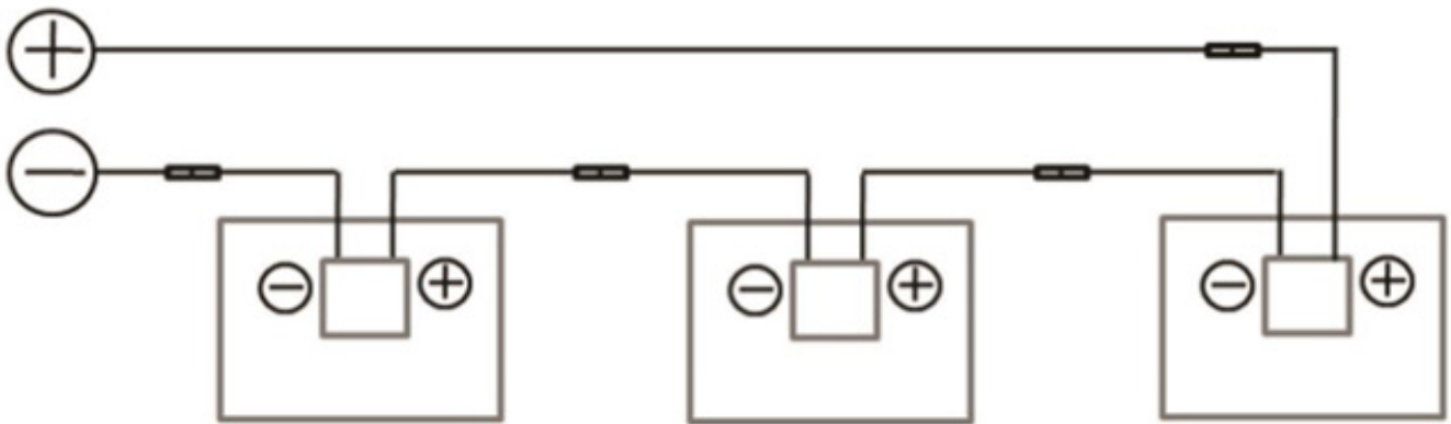
Series connection
