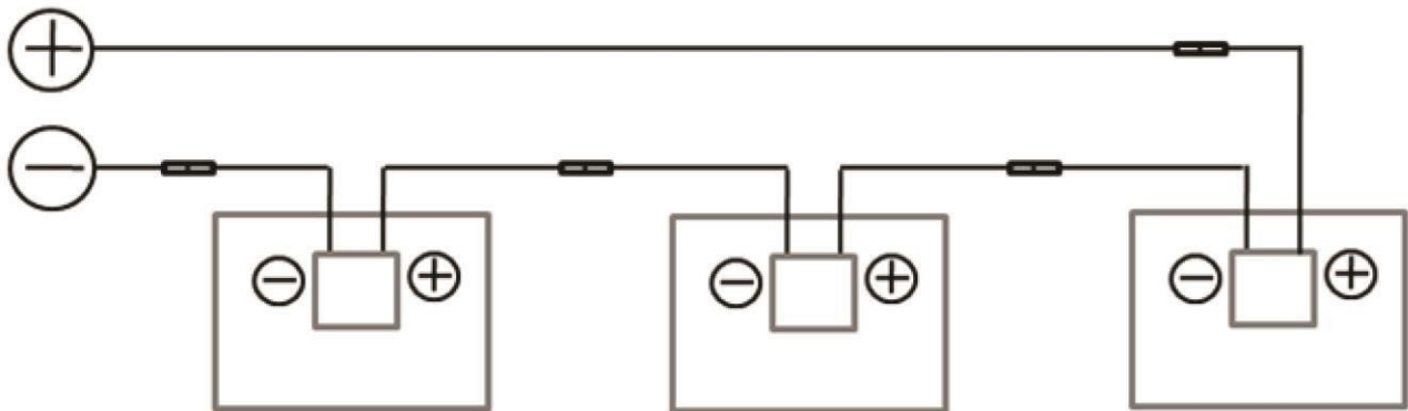
Series connection
